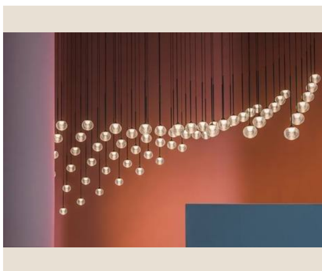
Algorithm Grid
